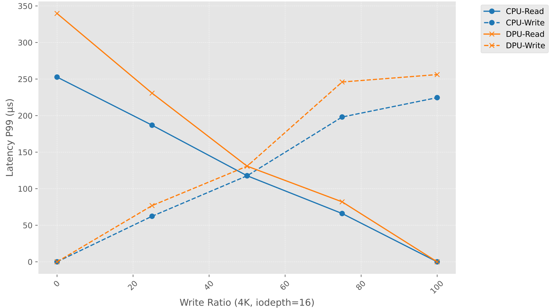
Latency P99 vs Write Ratio (4K, iodepth=16)
